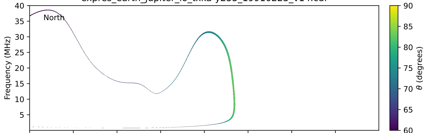
expres_earth_jupiter_io_txka-y235_19910223_v14.cdf
