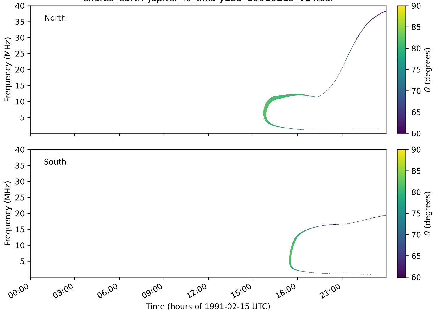
expres_earth_jupiter_io_txka-y235_19910215_v14.cdf
