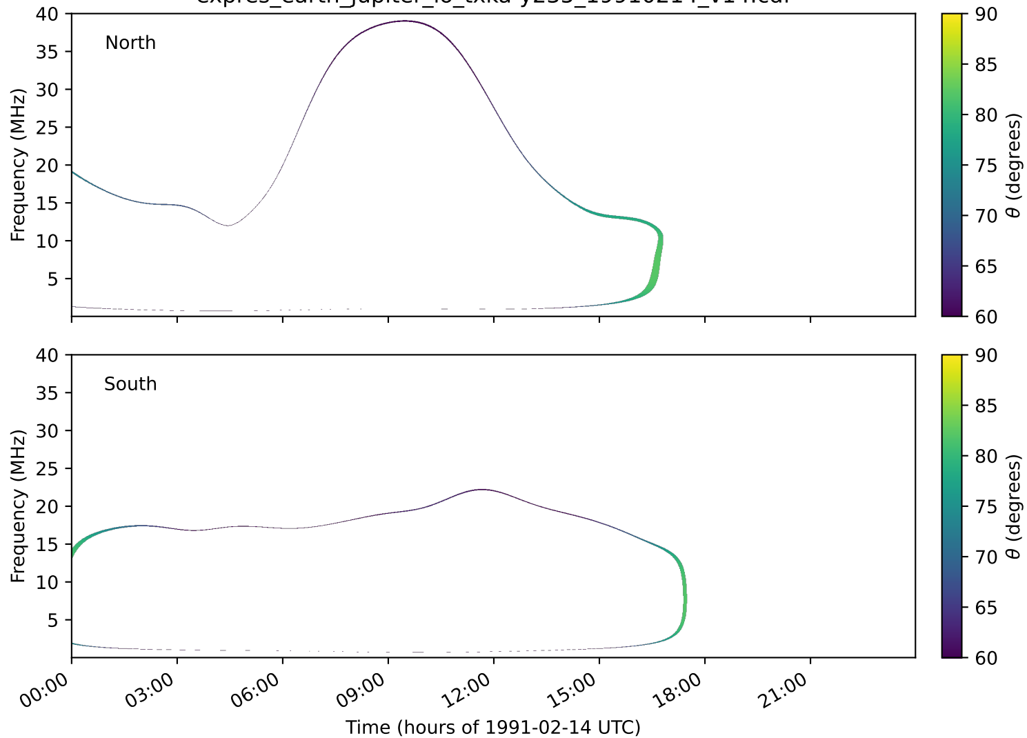
expres_earth_jupiter_io_txka-y235_19910214_v14.cdf
