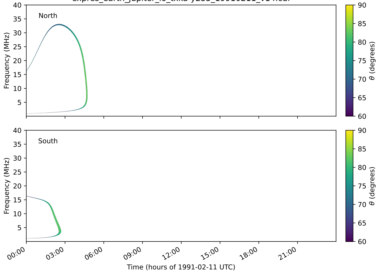
expres_earth_jupiter_io_txka-y235_19910211_v14.cdf
