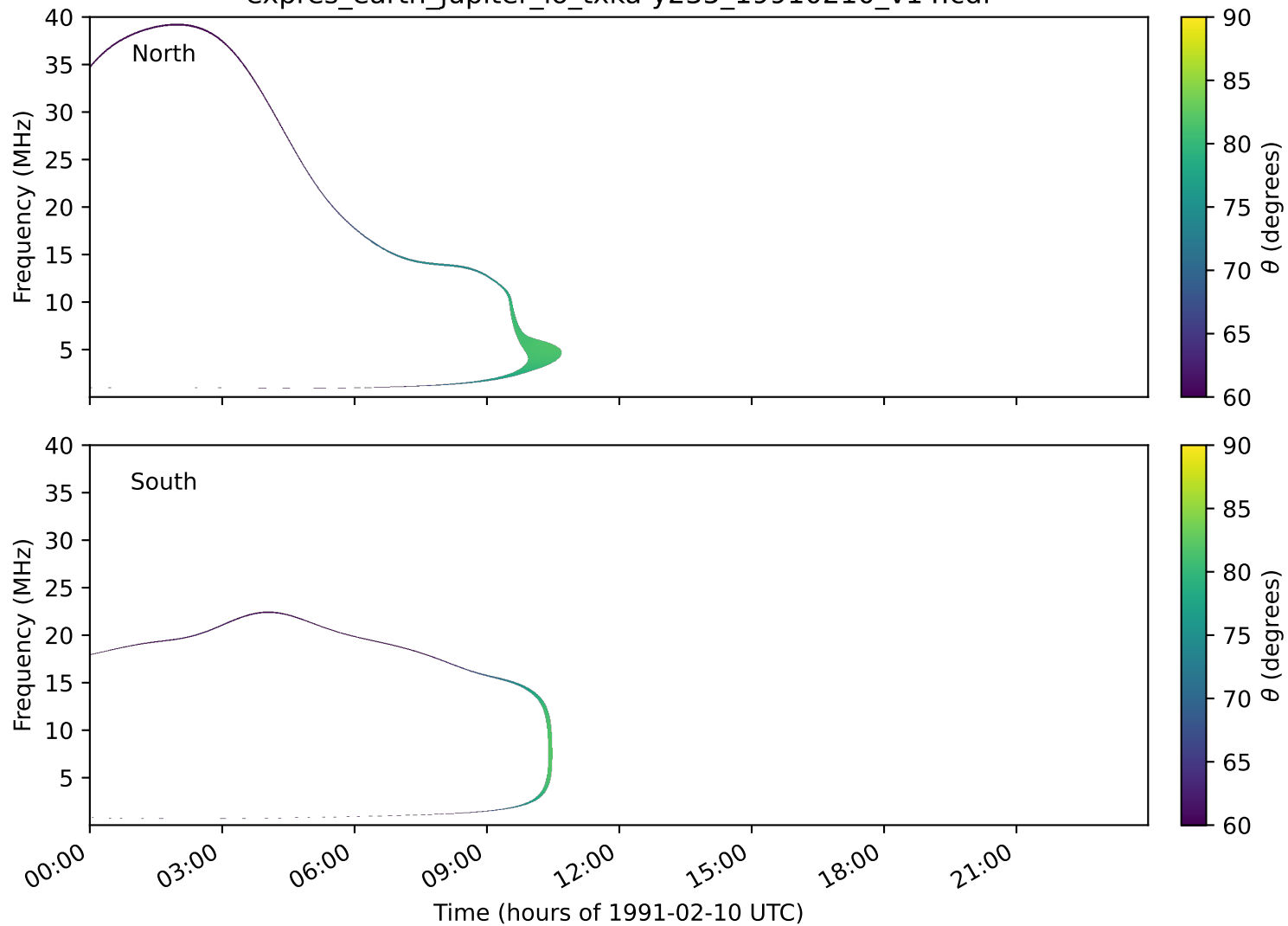
expres_earth_jupiter_io_txka-y235_19910210_v14.cdf
