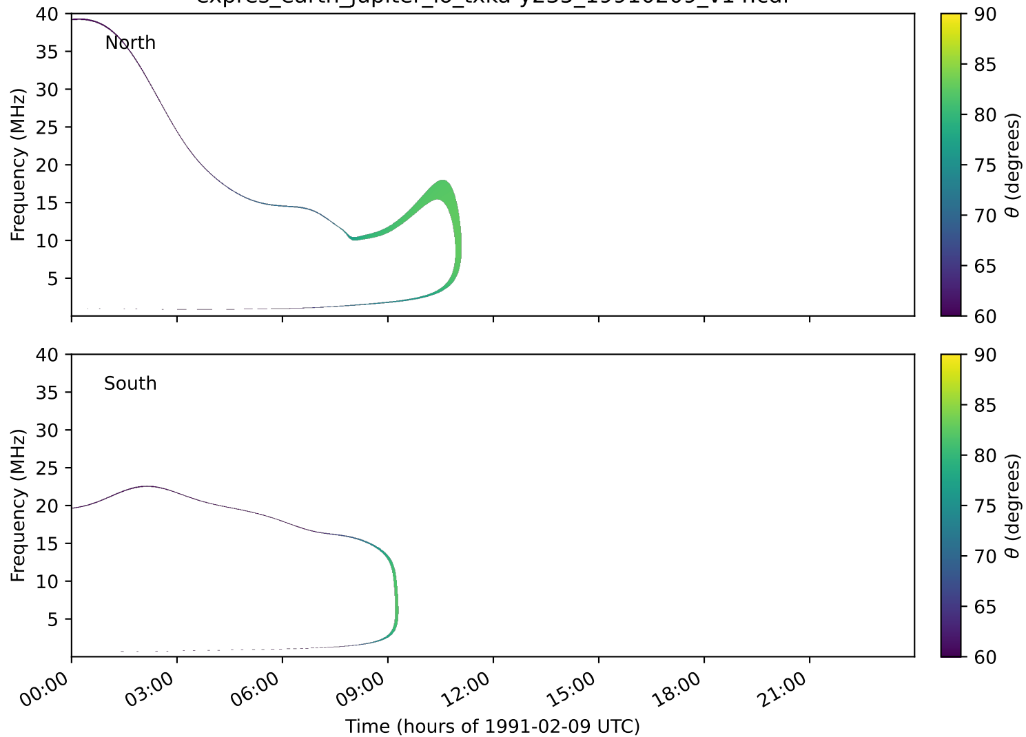
expres_earth_jupiter_io_txka-y235_19910209_v14.cdf
