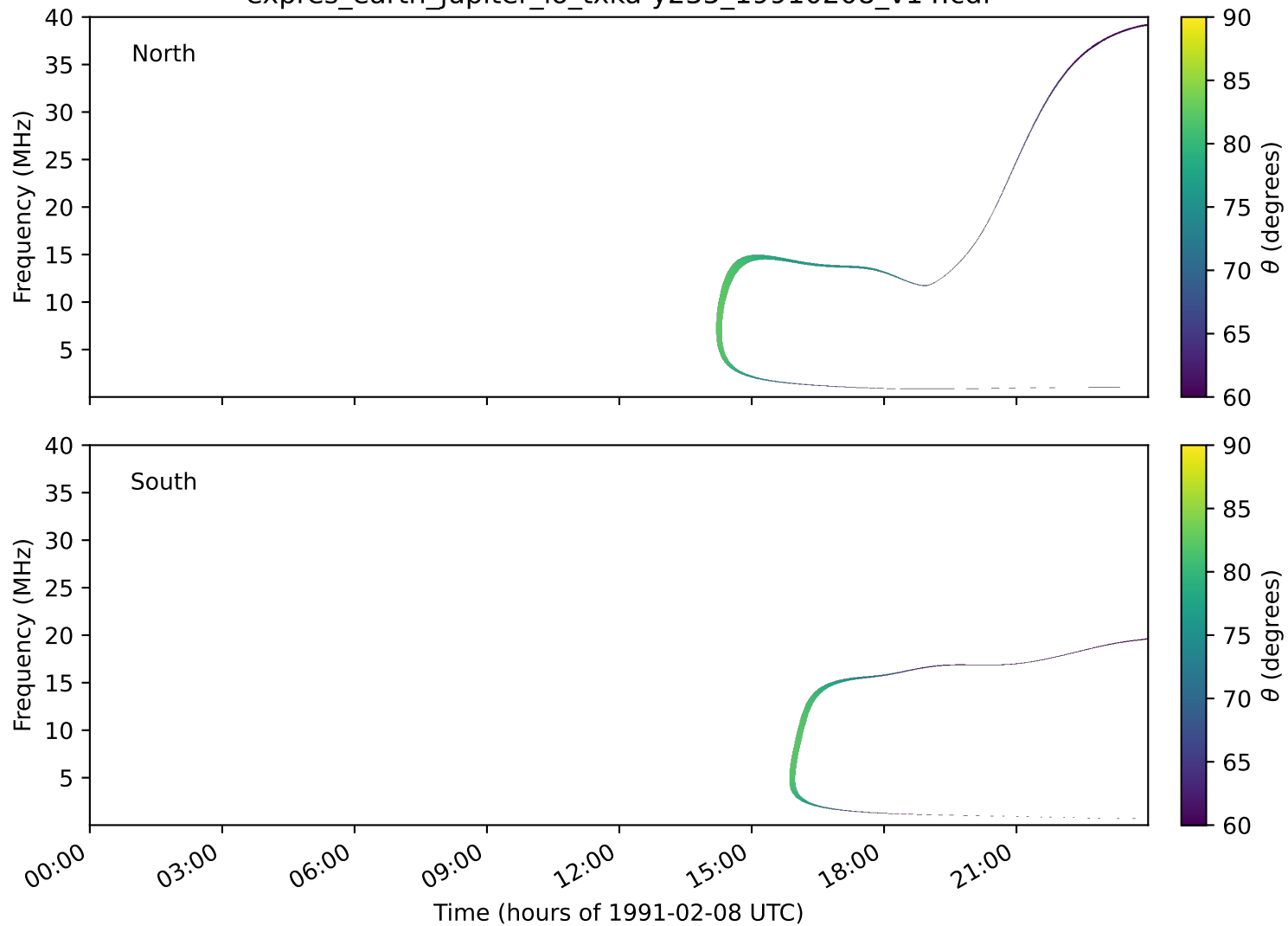
expres_earth_jupiter_io_txka-y235_19910208_v14.cdf
