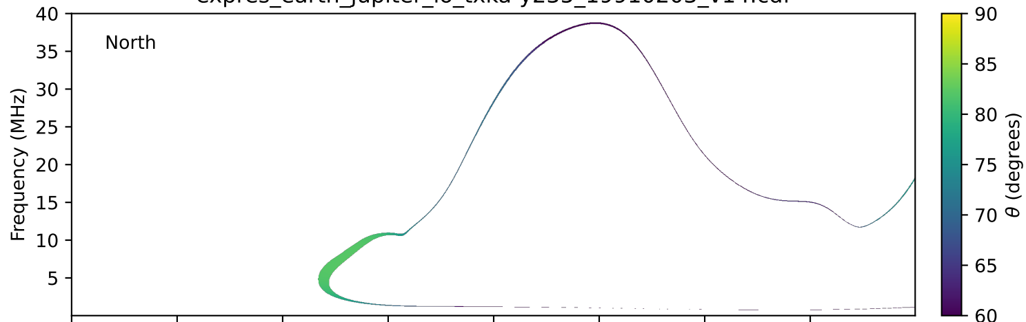
expres_earth_jupiter_io_txka-y235_19910203_v14.cdf
