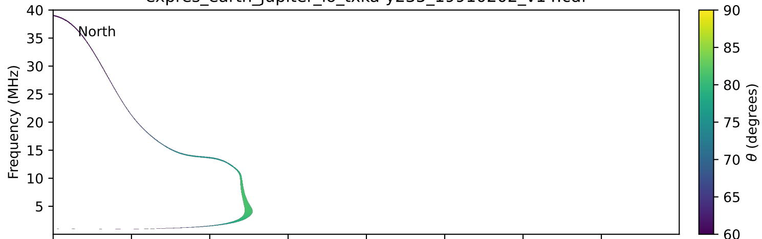
expres_earth_jupiter_io_txka-y235_19910202_v14.cdf
