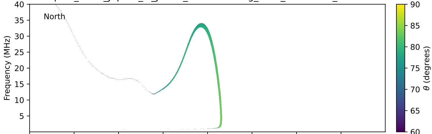
expres_earth_jupiter_io_jrm33_lossc-wid1deg_3kev_19910216_v11.cdf
