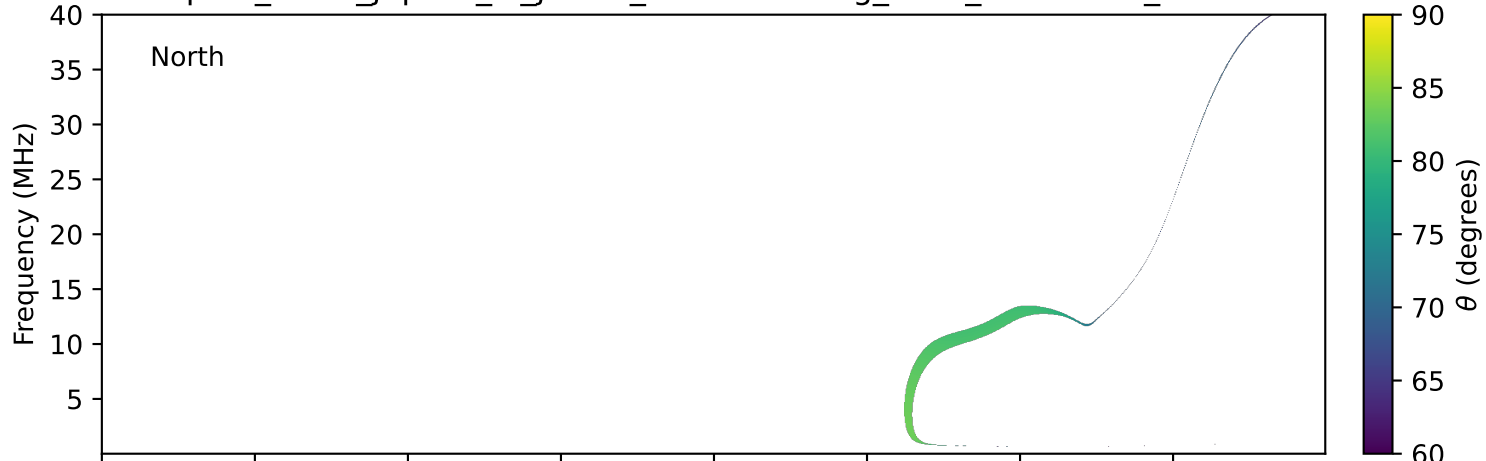
expres_earth_jupiter_io_jrm33_lossc-wid1deg_3kev_19910215_v11.cdf
