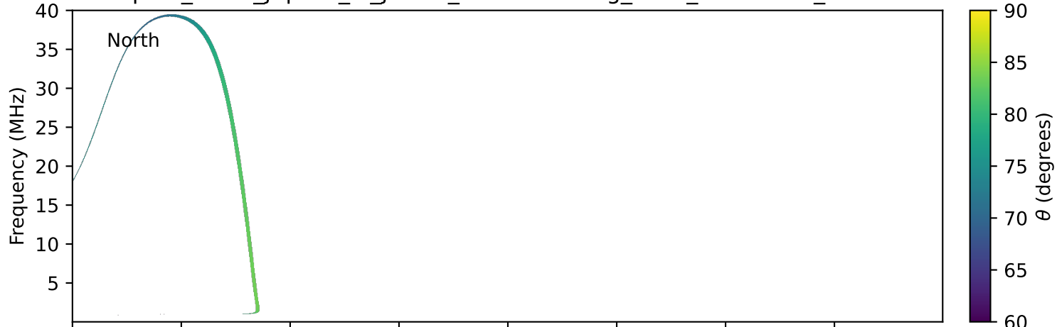
expres_earth_jupiter_io_jrm33_lossc-wid1deg_3kev_19910211_v11.cdf
