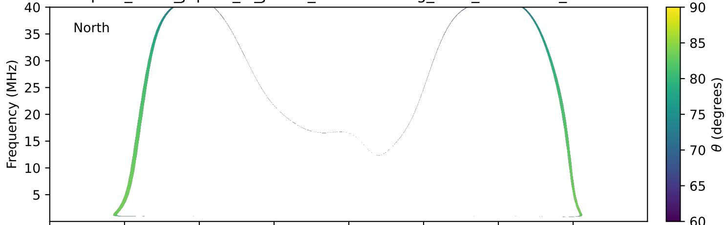
expres_earth_jupiter_io_jrm33_lossc-wid1deg_3kev_19910205_v11.cdf
