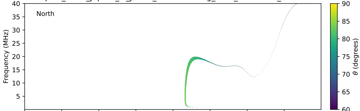
expres_earth_jupiter_io_jrm33_lossc-wid1deg_3kev_19910201_v11.cdf
