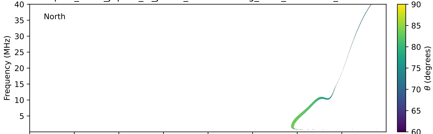
expres_earth_jupiter_io_jrm09_lossc-wid1deg_3kev_19910222_v11.cdf
