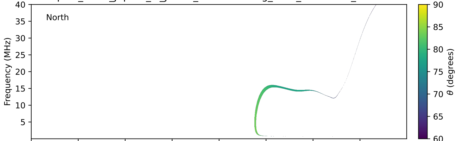
expres_earth_jupiter_io_jrm09_lossc-wid1deg_3kev_19910208_v11.cdf
