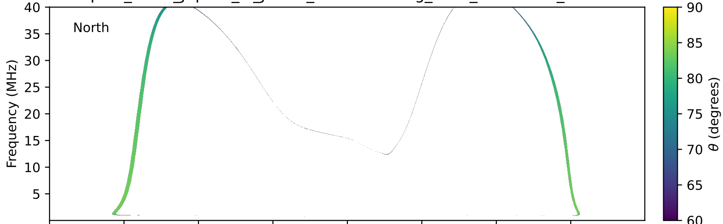
expres_earth_jupiter_io_jrm09_lossc-wid1deg_3kev_19910205_v11.cdf
