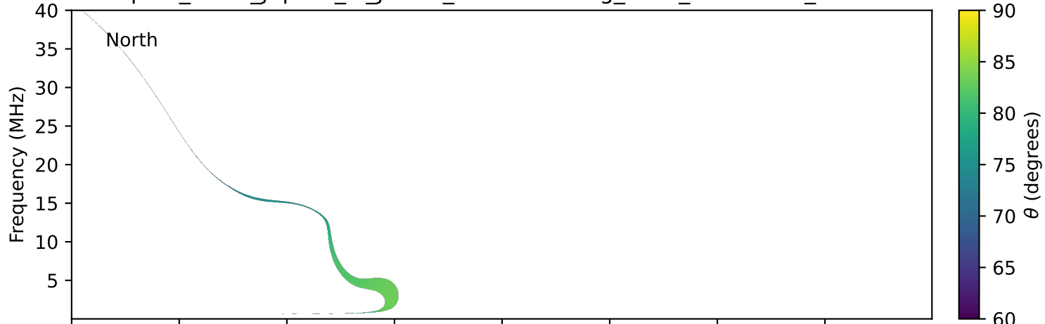
expres_earth_jupiter_io_jrm09_lossc-wid1deg_3kev_19910202_v11.cdf
