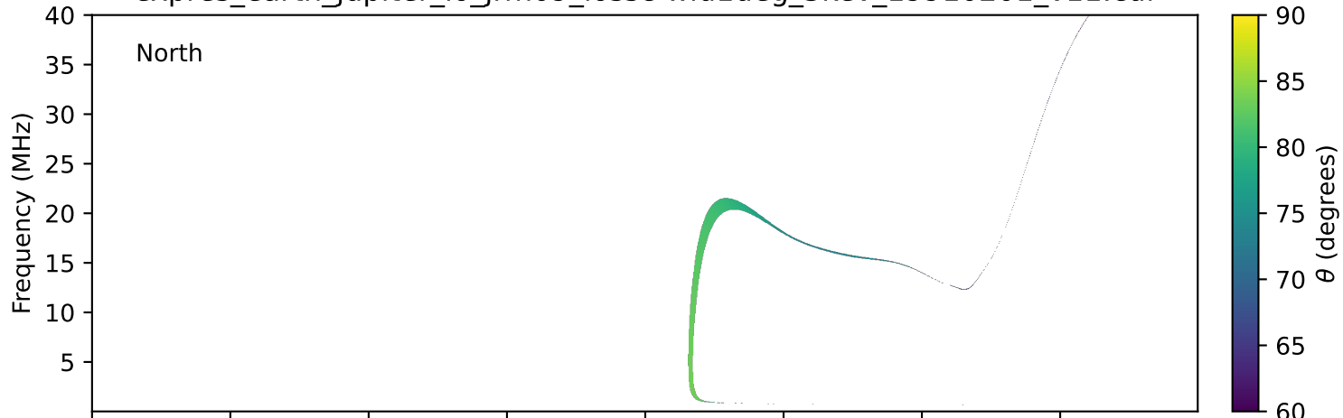
expres_earth_jupiter_io_jrm09_lossc-wid1deg_3kev_19910201_v11.cdf
