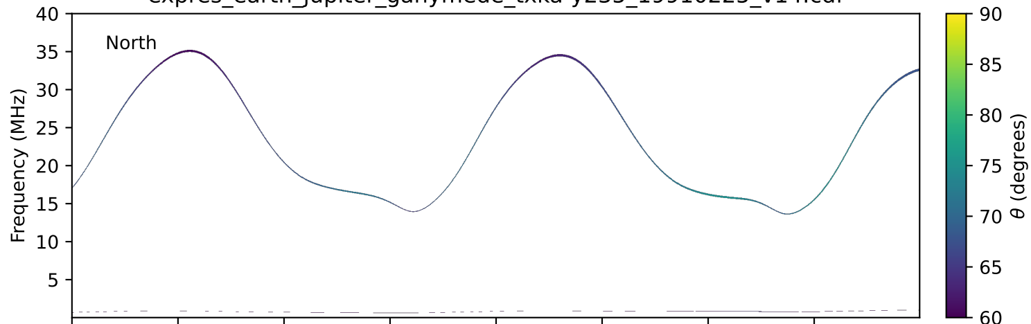
expres_earth_jupiter_ganymede_txka-y235_19910225_v14.cdf
