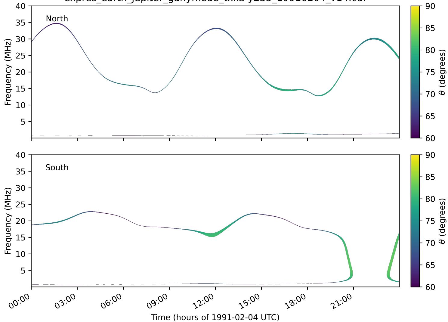
expres_earth_jupiter_ganymede_txka-y235_19910204_v14.cdf
