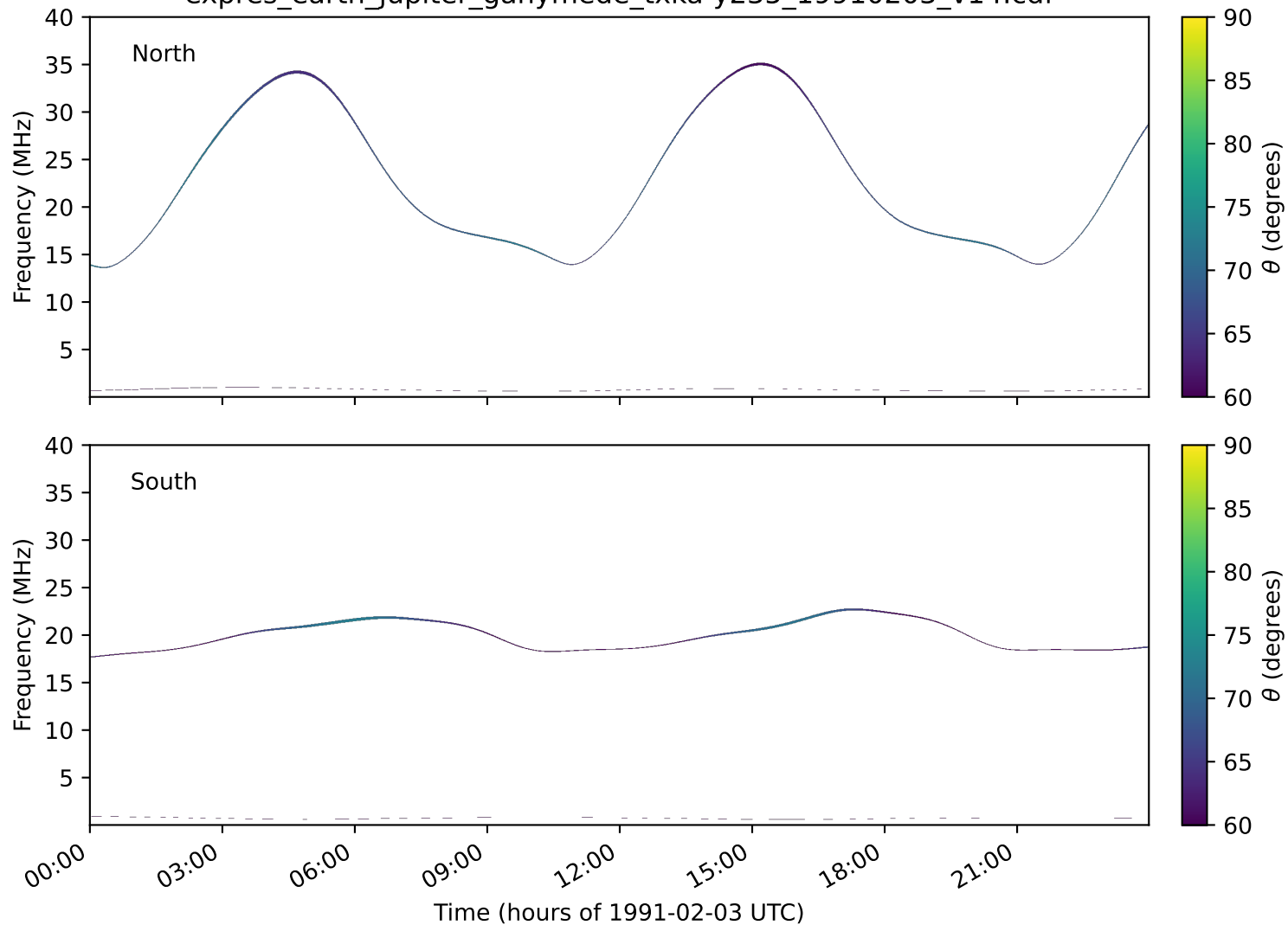
expres_earth_jupiter_ganymede_txka-y235_19910203_v14.cdf
