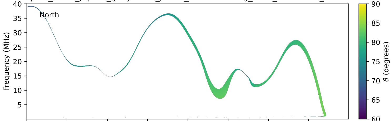
expres_earth_jupiter_ganymede_jrm33_lossc-wid1deg_3kev_19910226_v11.cdf
