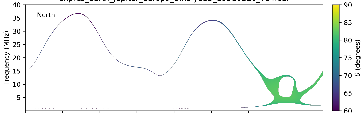
expres_earth_jupiter_europa_txka-y235_19910220_v14.cdf
