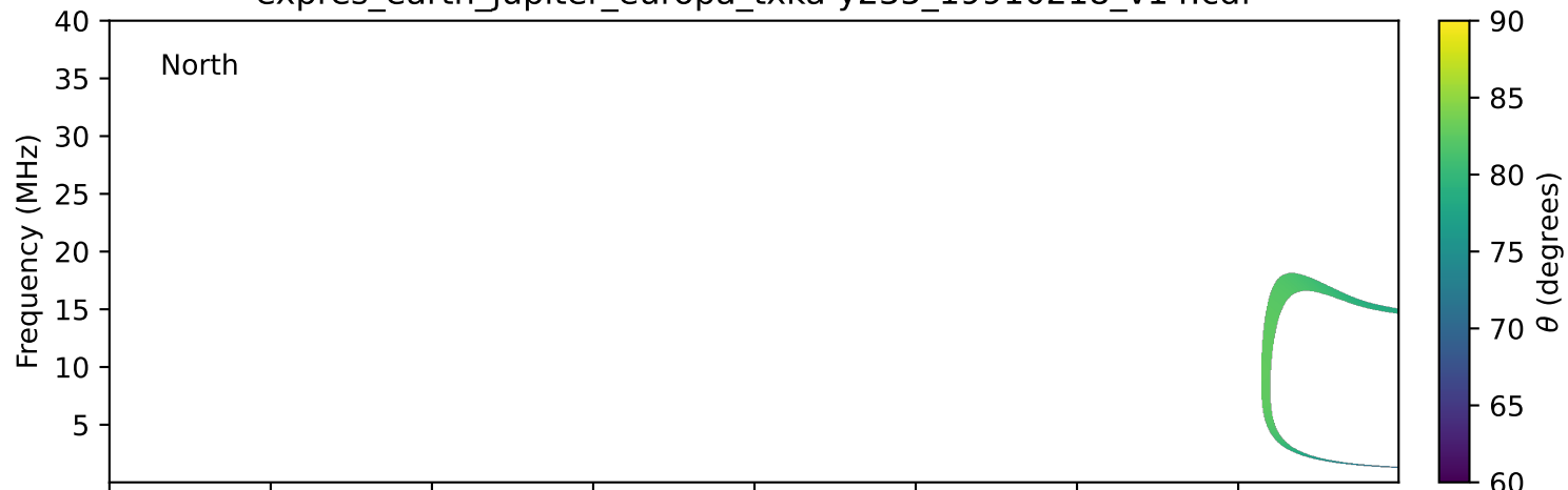
expres_earth_jupiter_europa_txka-y235_19910218_v14.cdf
