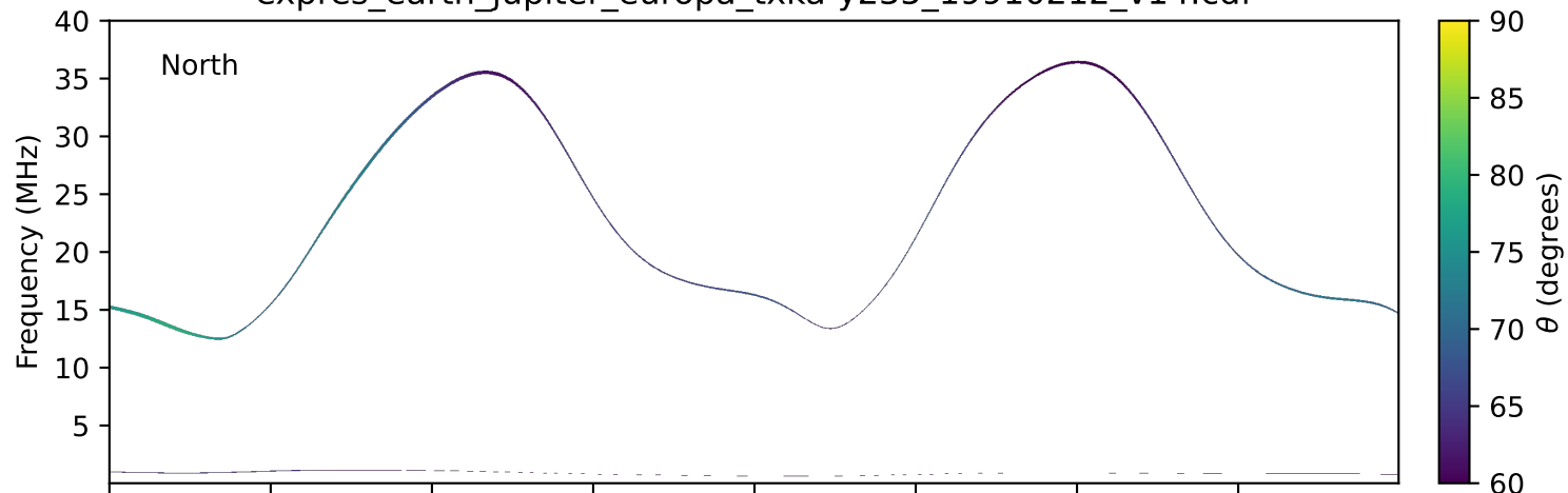
expres_earth_jupiter_europa_txka-y235_19910212_v14.cdf
