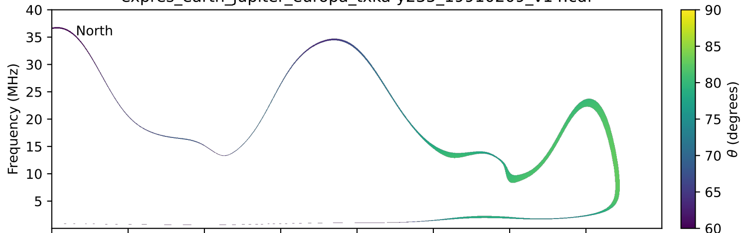
expres_earth_jupiter_europa_txka-y235_19910209_v14.cdf
