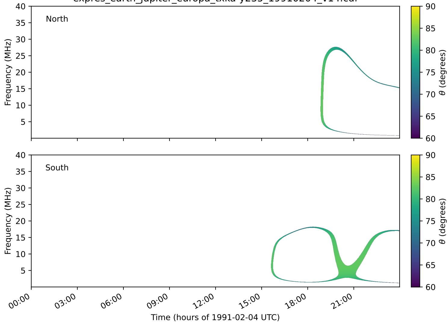
expres_earth_jupiter_europa_txka-y235_19910204_v14.cdf
