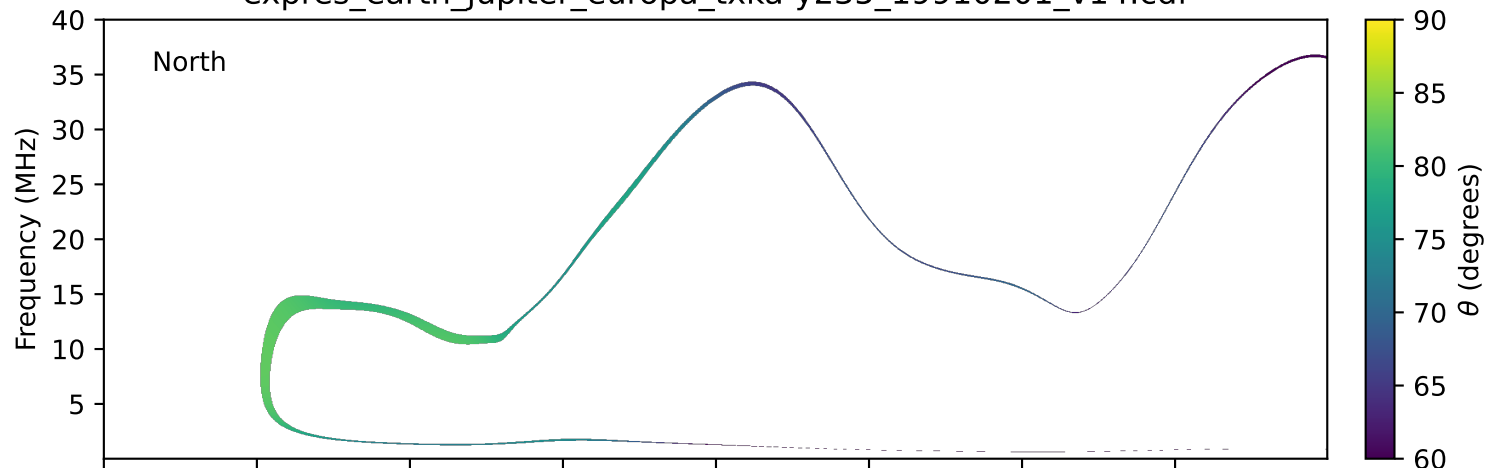
expres_earth_jupiter_europa_txka-y235_19910201_v14.cdf
