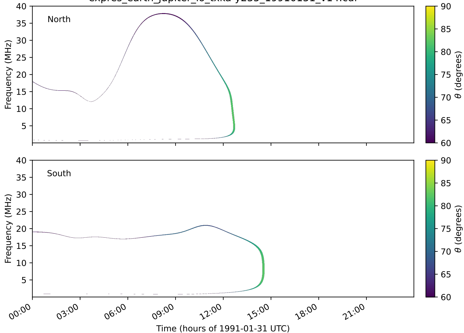
expres_earth_jupiter_io_txka-y235_19910131_v14.cdf
