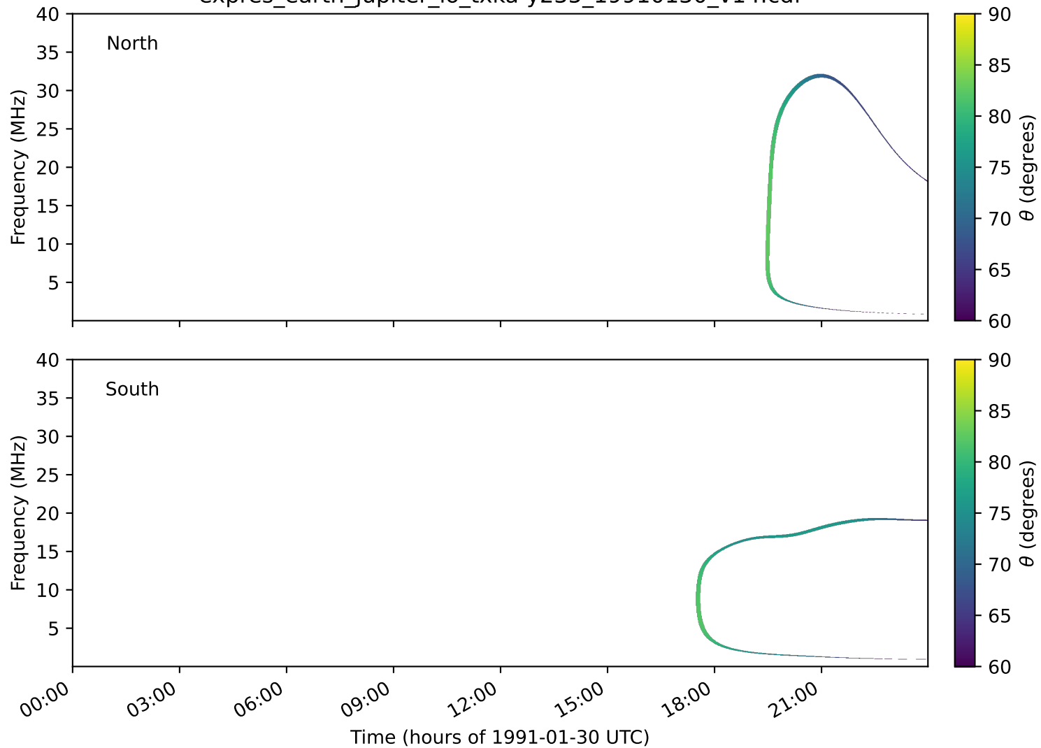
expres_earth_jupiter_io_txka-y235_19910130_v14.cdf
