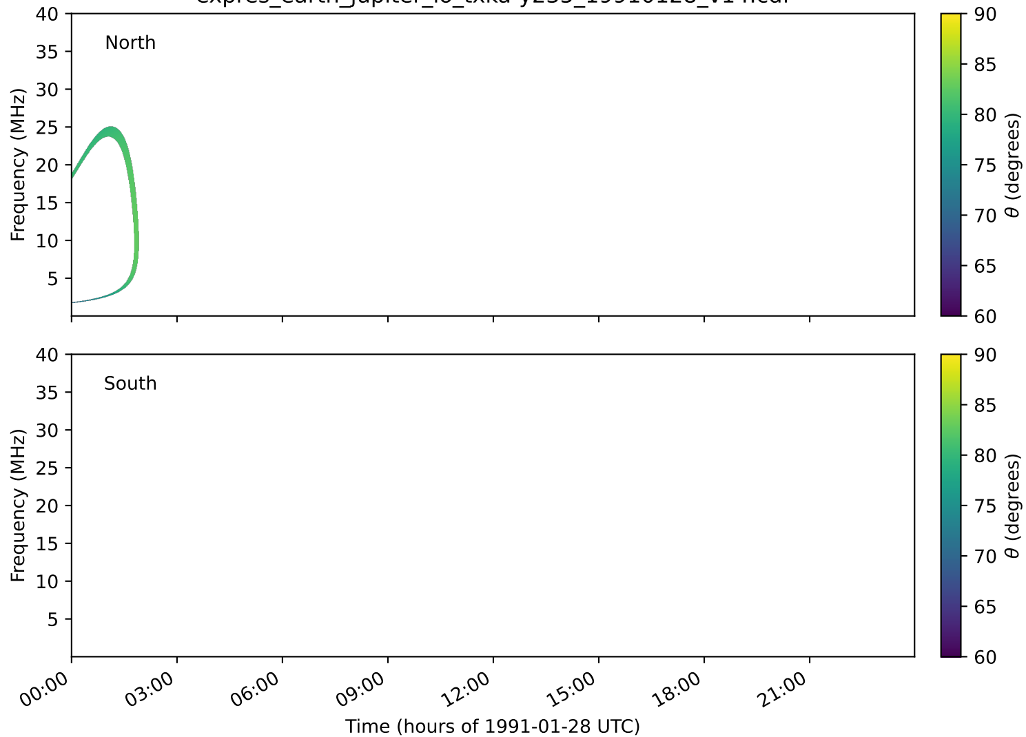
expres_earth_jupiter_io_txka-y235_19910128_v14.cdf
