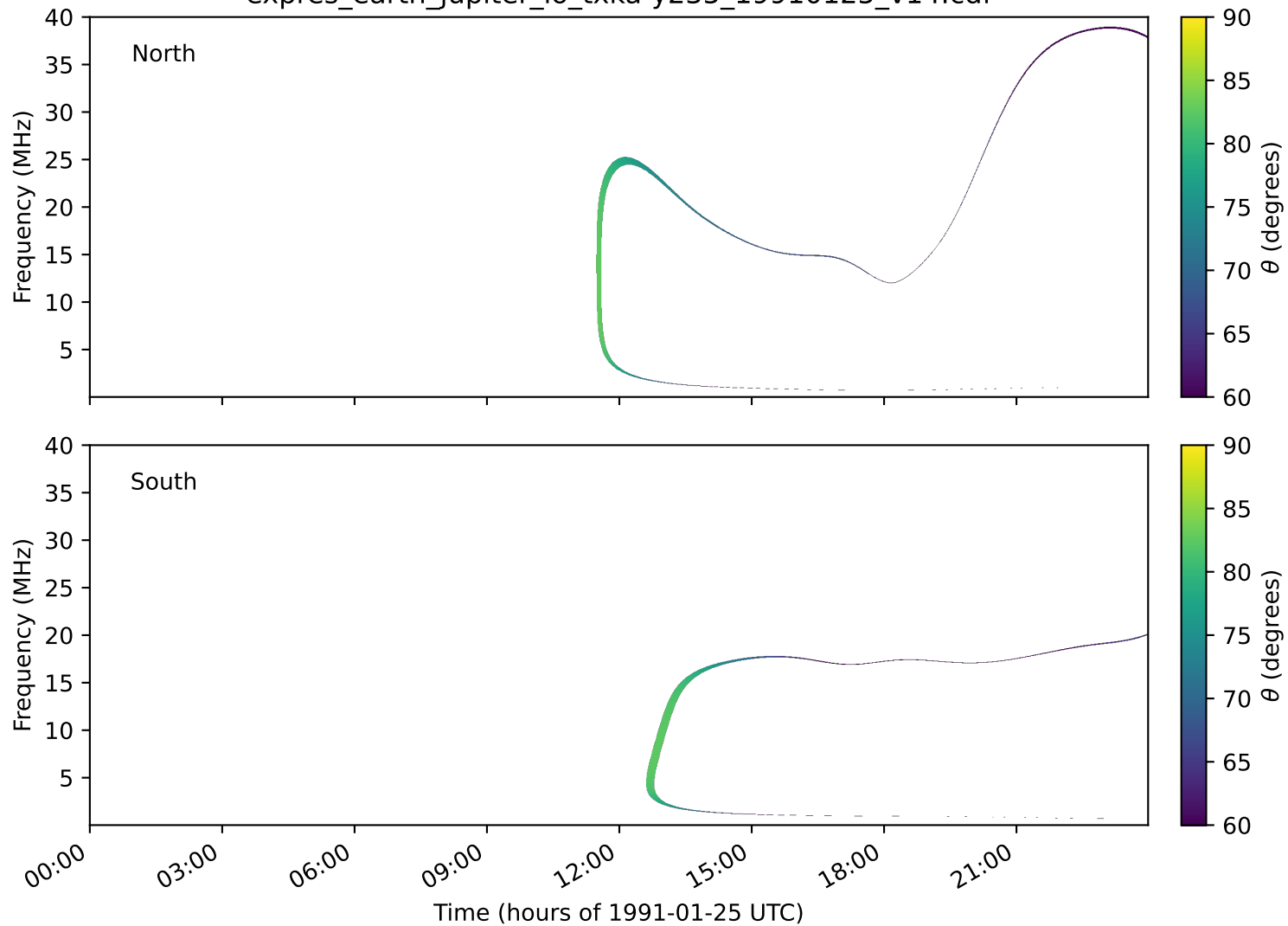
expres_earth_jupiter_io_txka-y235_19910125_v14.cdf
