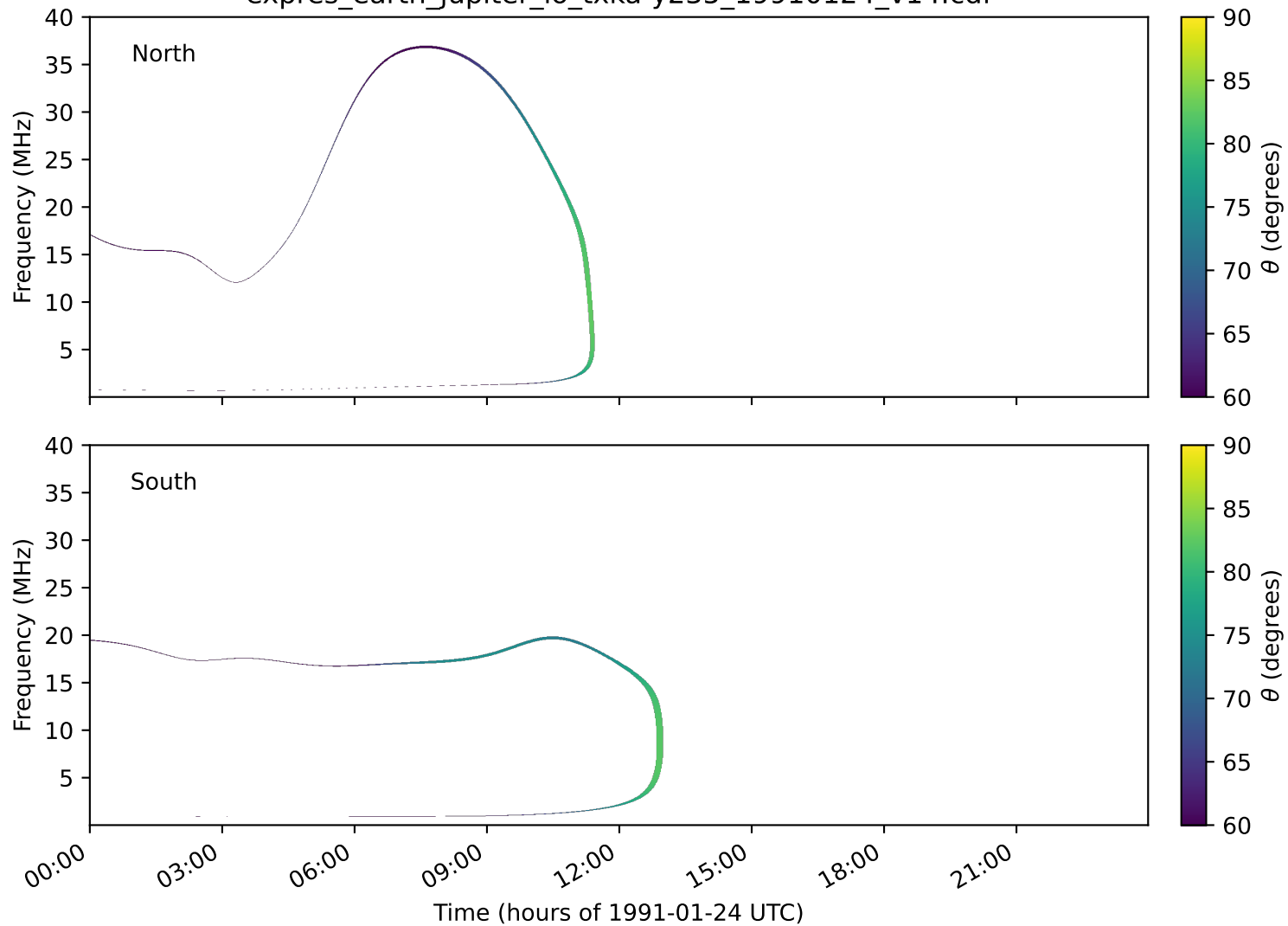
expres_earth_jupiter_io_txka-y235_19910124_v14.cdf
