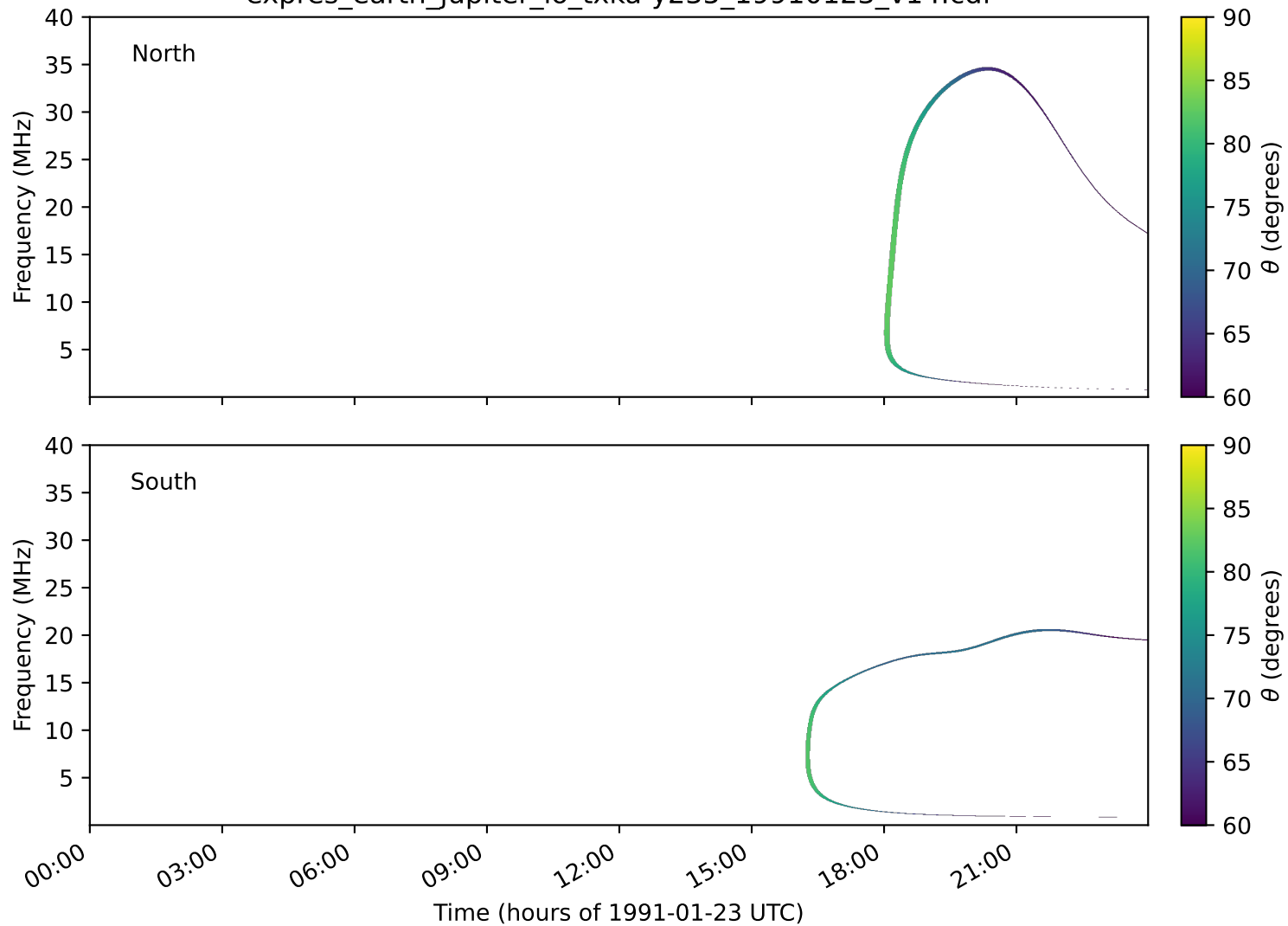
expres_earth_jupiter_io_txka-y235_19910123_v14.cdf
