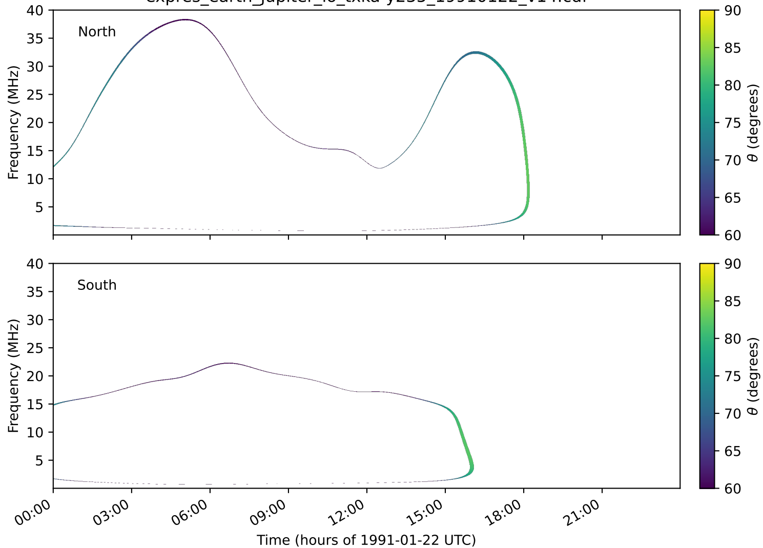
expres_earth_jupiter_io_txka-y235_19910122_v14.cdf
