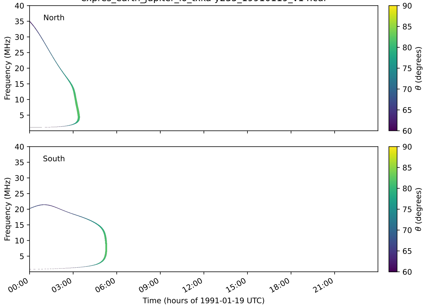
expres_earth_jupiter_io_txka-y235_19910119_v14.cdf
