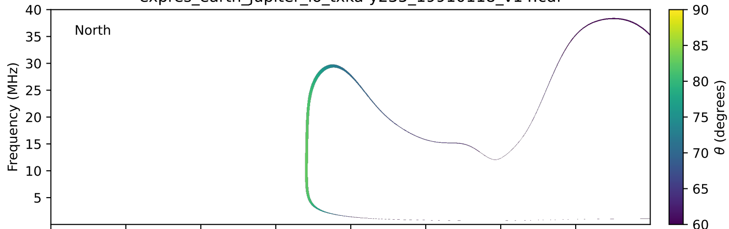
expres_earth_jupiter_io_txka-y235_19910118_v14.cdf
