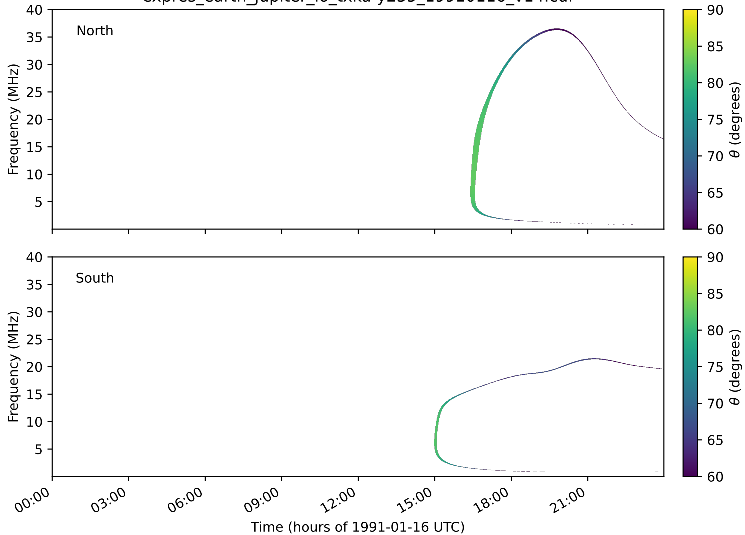
expres_earth_jupiter_io_txka-y235_19910116_v14.cdf
