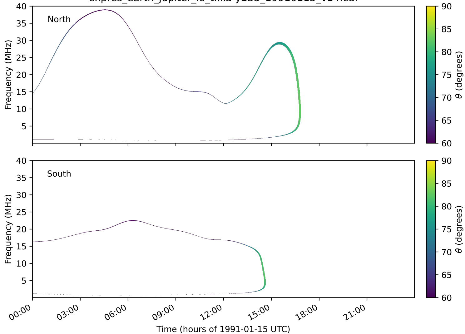
expres_earth_jupiter_io_txka-y235_19910115_v14.cdf
