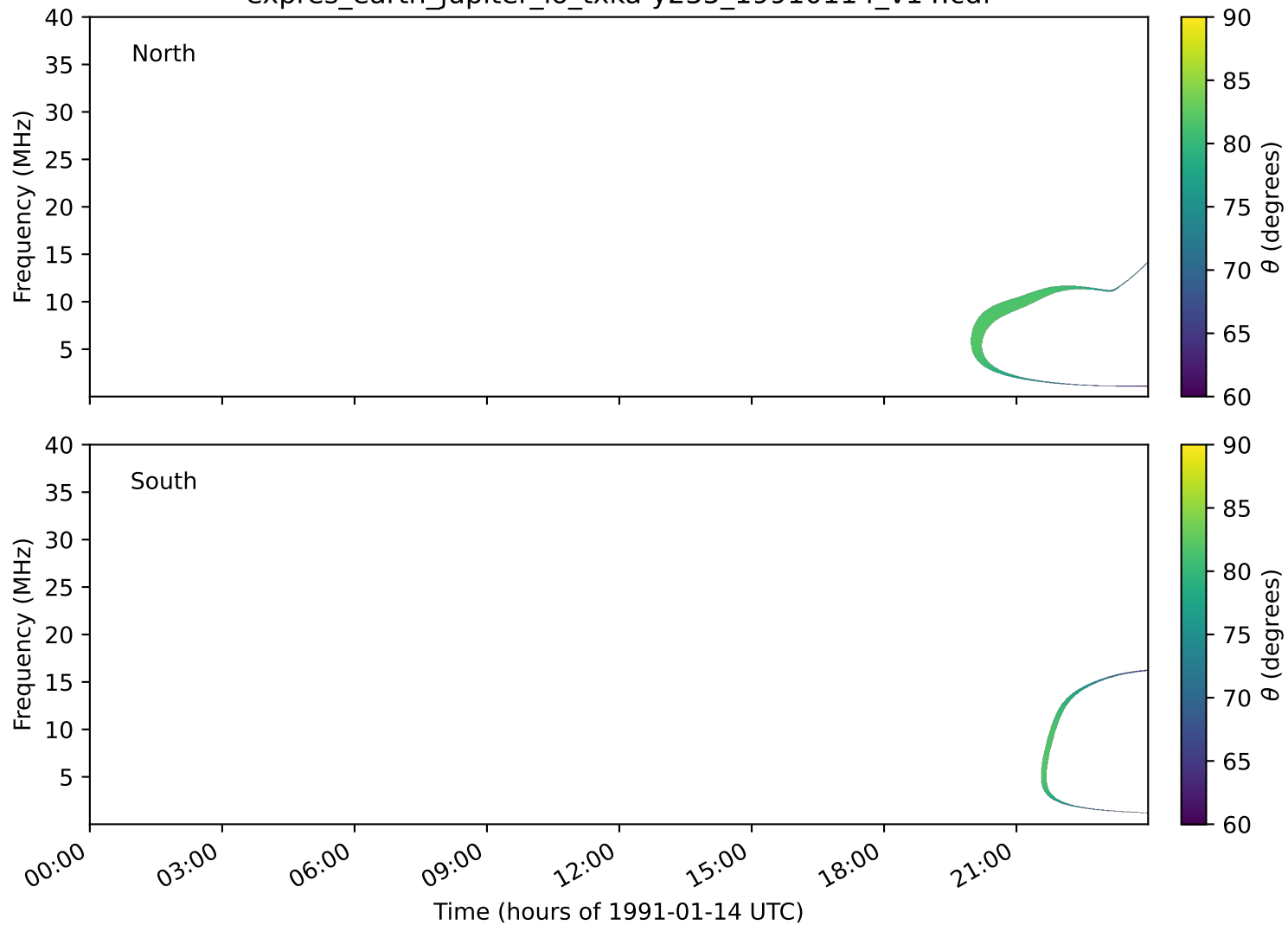
expres_earth_jupiter_io_txka-y235_19910114_v14.cdf
