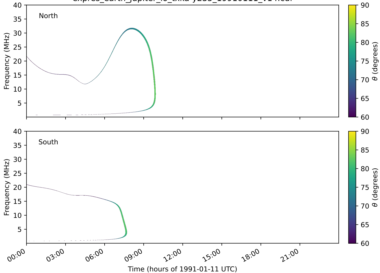
expres_earth_jupiter_io_txka-y235_19910111_v14.cdf
