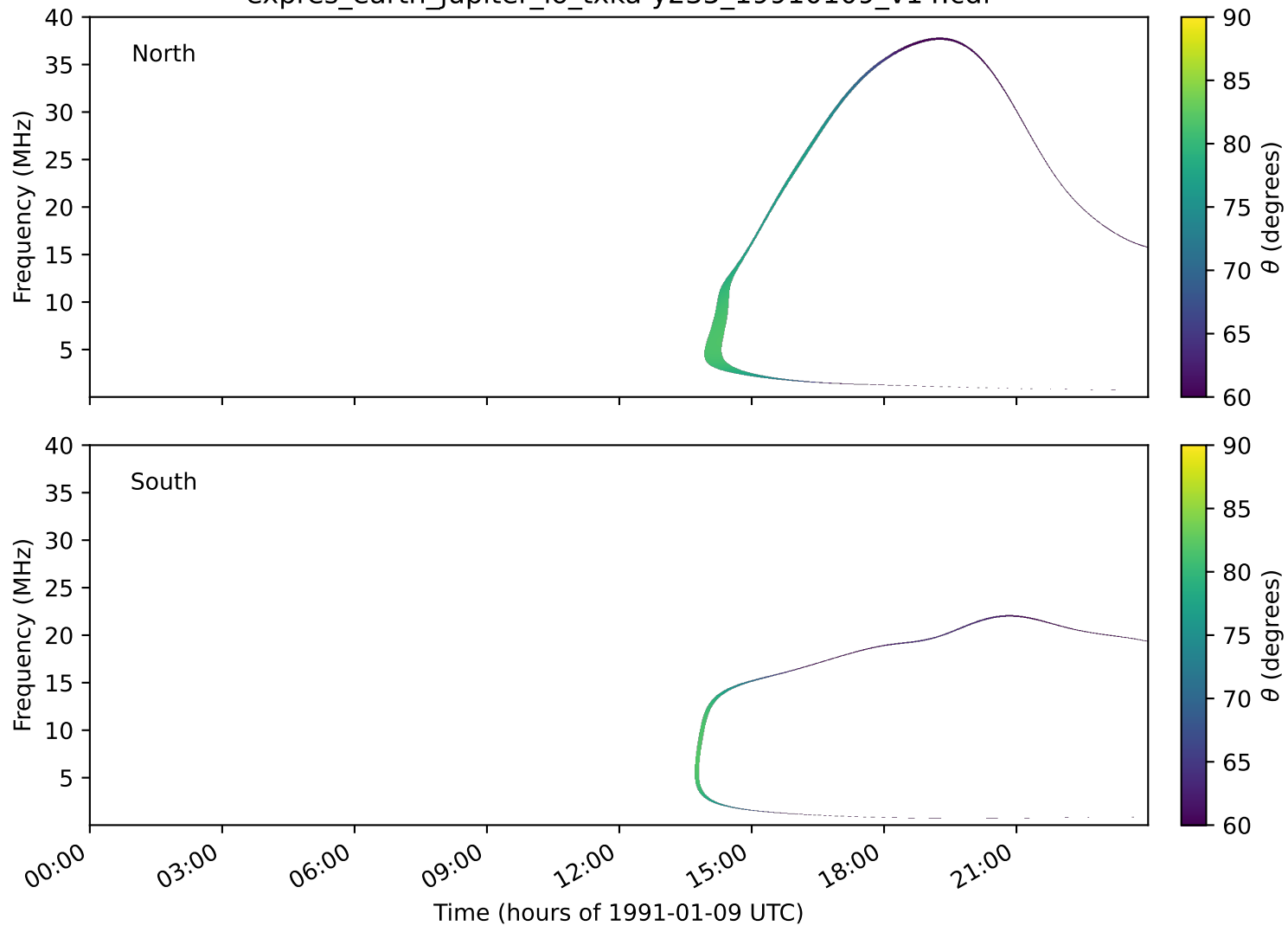
expres_earth_jupiter_io_txka-y235_19910109_v14.cdf
