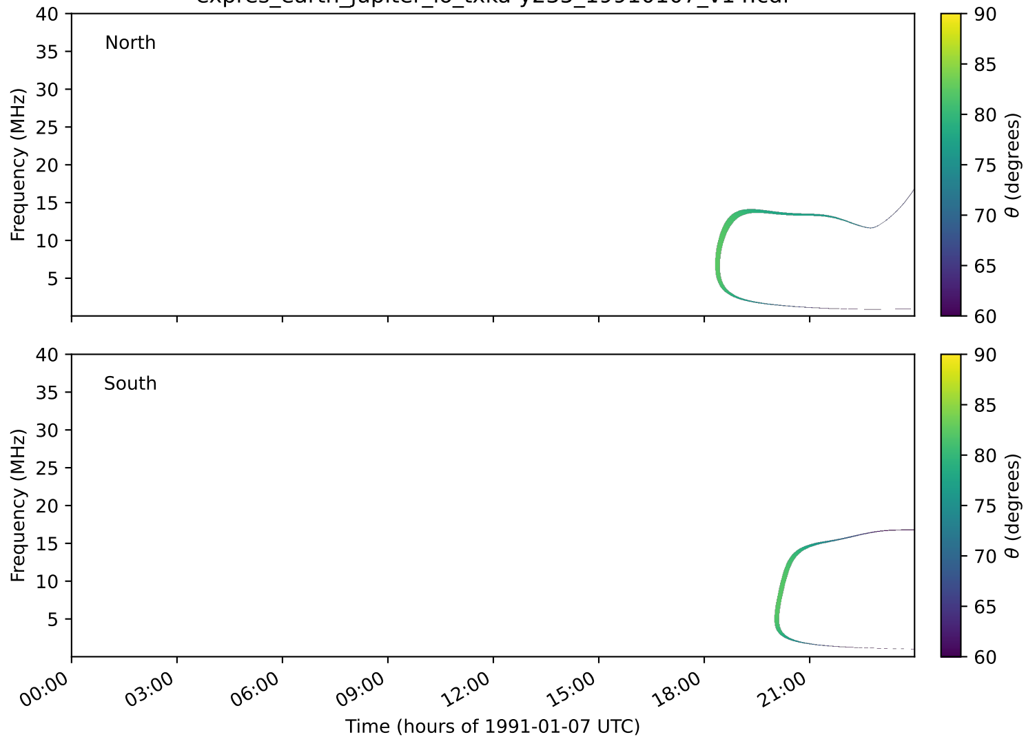
expres_earth_jupiter_io_txka-y235_19910107_v14.cdf
