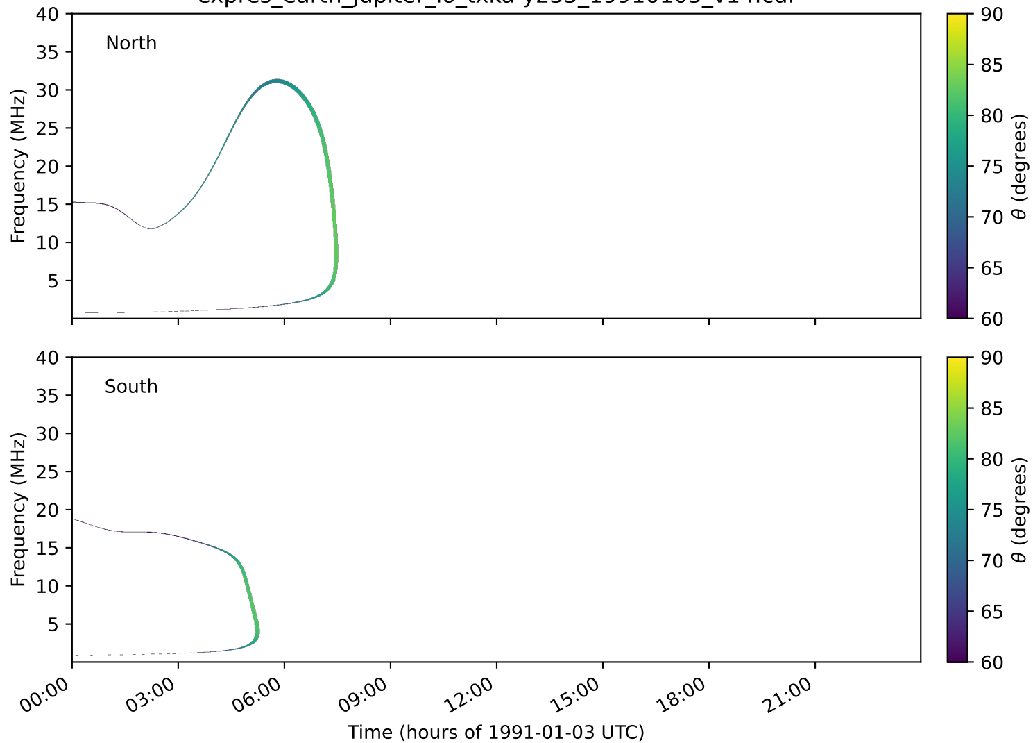
expres_earth_jupiter_io_txka-y235_19910103_v14.cdf
