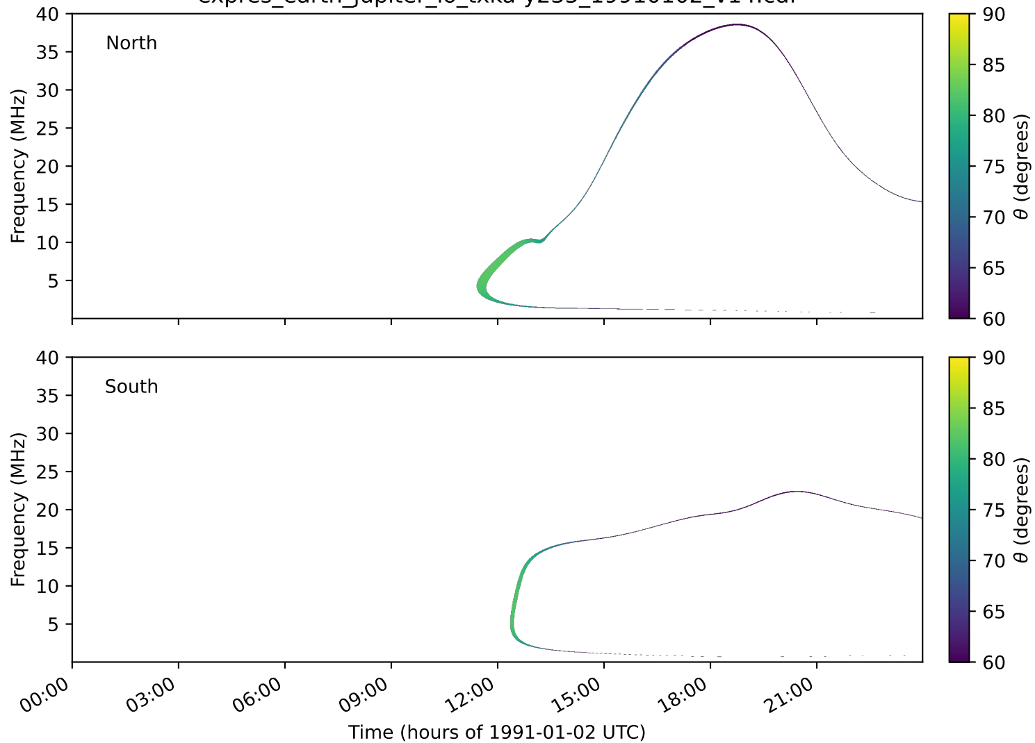
expres_earth_jupiter_io_txka-y235_19910102_v14.cdf
