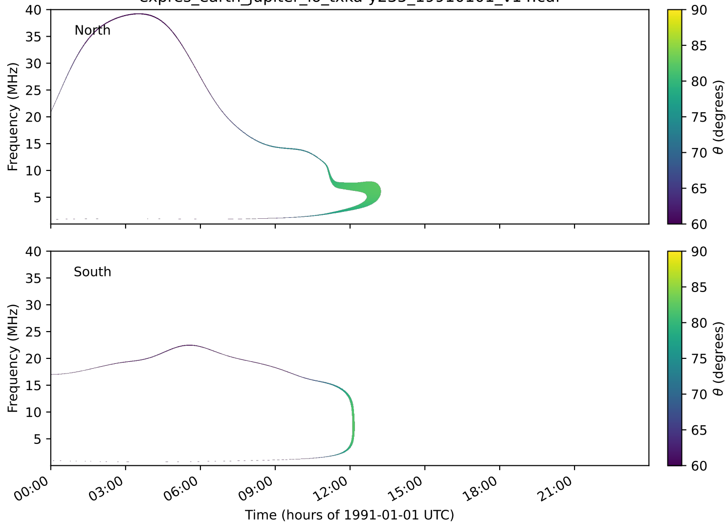
expres_earth_jupiter_io_txka-y235_19910101_v14.cdf
