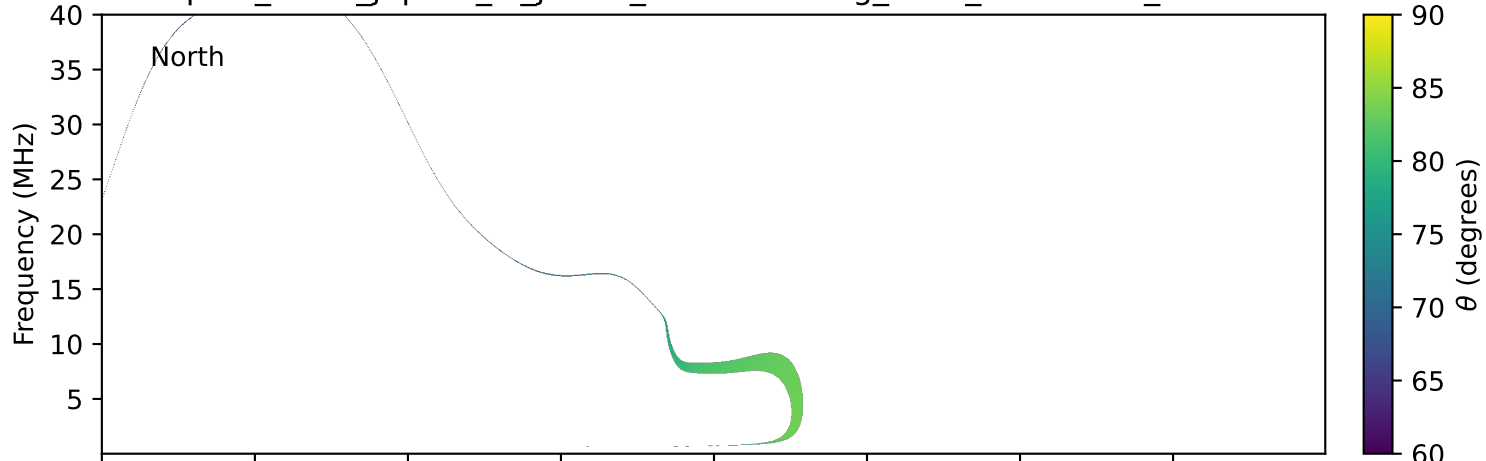
expres_earth_jupiter_io_jrm33_lossc-wid1deg_3kev_19910101_v11.cdf
