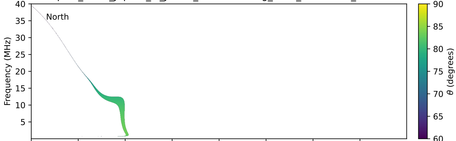
expres_earth_jupiter_io_jrm09_lossc-wid1deg_3kev_19910126_v11.cdf
