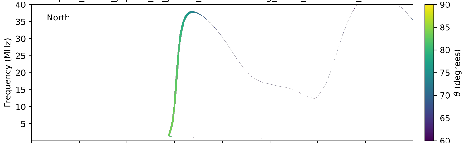
expres_earth_jupiter_io_jrm09_lossc-wid1deg_3kev_19910111_v11.cdf
